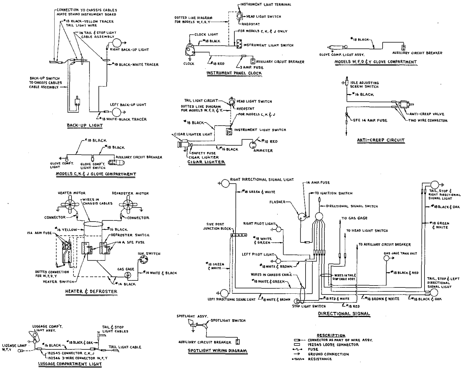
FIG. 2 AUXILIARY WIRING DIAGRAM
