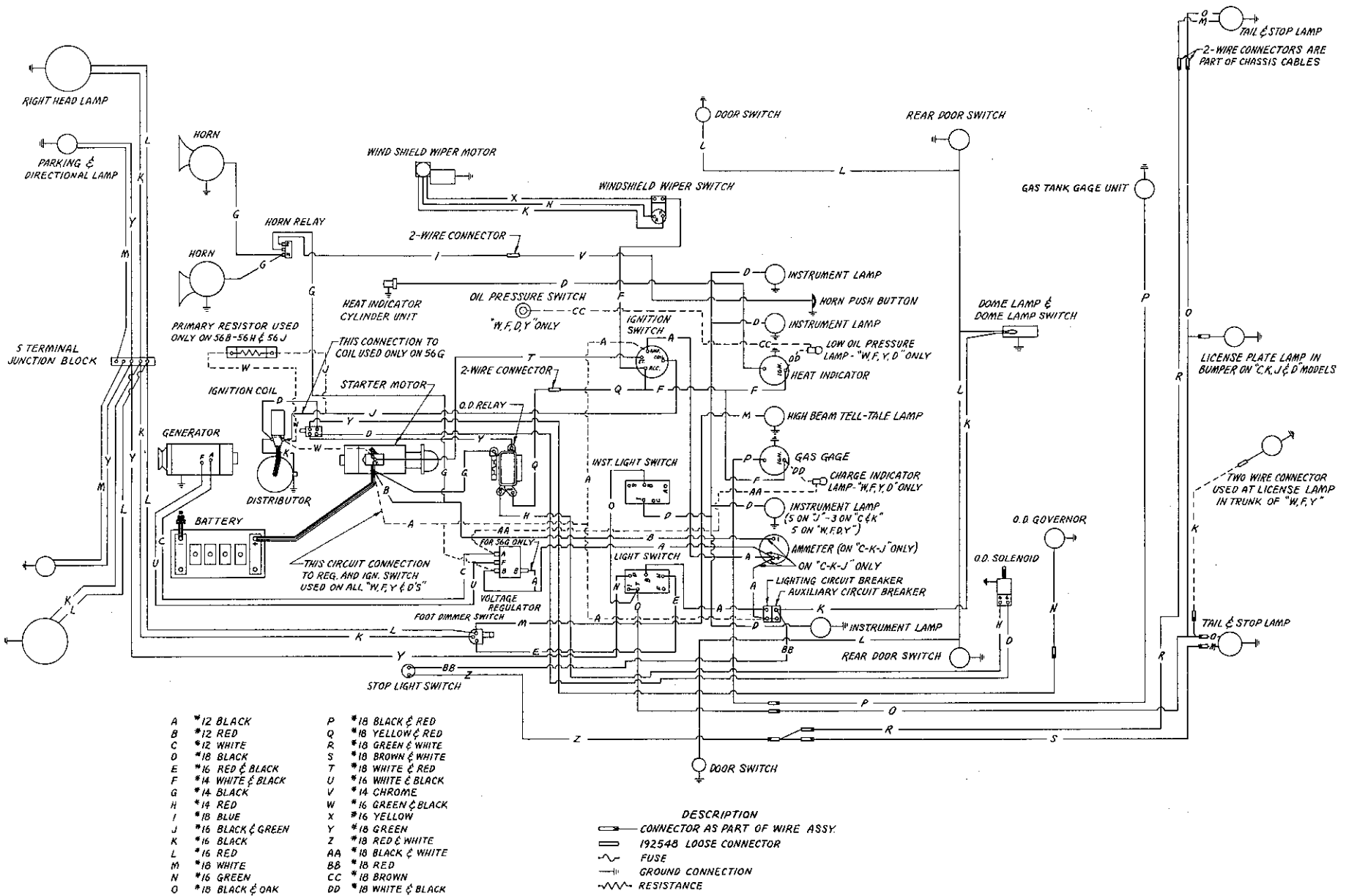
FIG. 1 MAIN WIRING DIAGRAM
